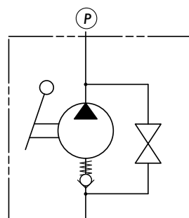
WITH VALVE
