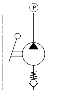
WITHOUT VALVE
